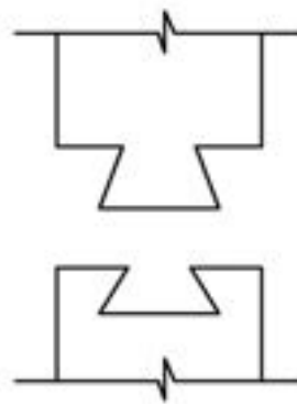
Fig. 24: Dovetail joint
