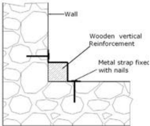
Fig. 21: Vertical Reinforcement at Corner
